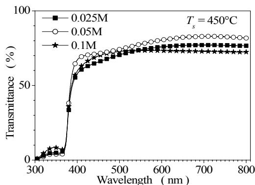
Fig. 4 Variation of the optical transmittance with the wavelength for different molarities at 450°C.
